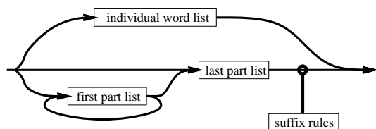
Figure 1: Look-up scheme for compound splitting.
